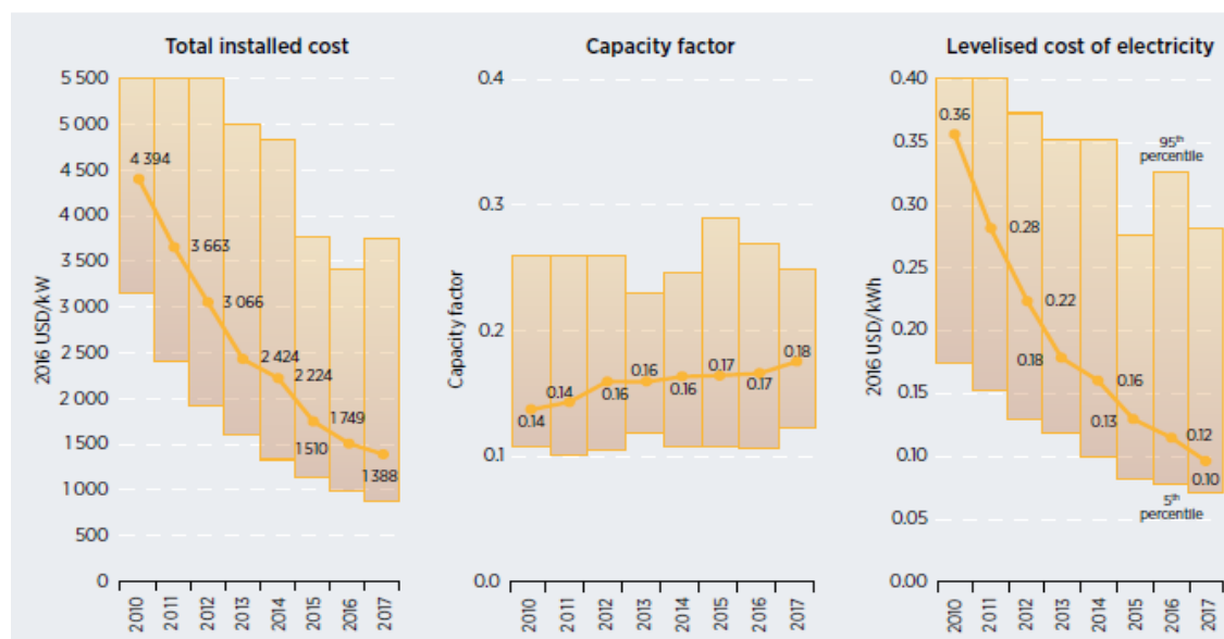
Figure 12: Example of decreasing renewable energy source costs (source: Irena 31 , 2017)
