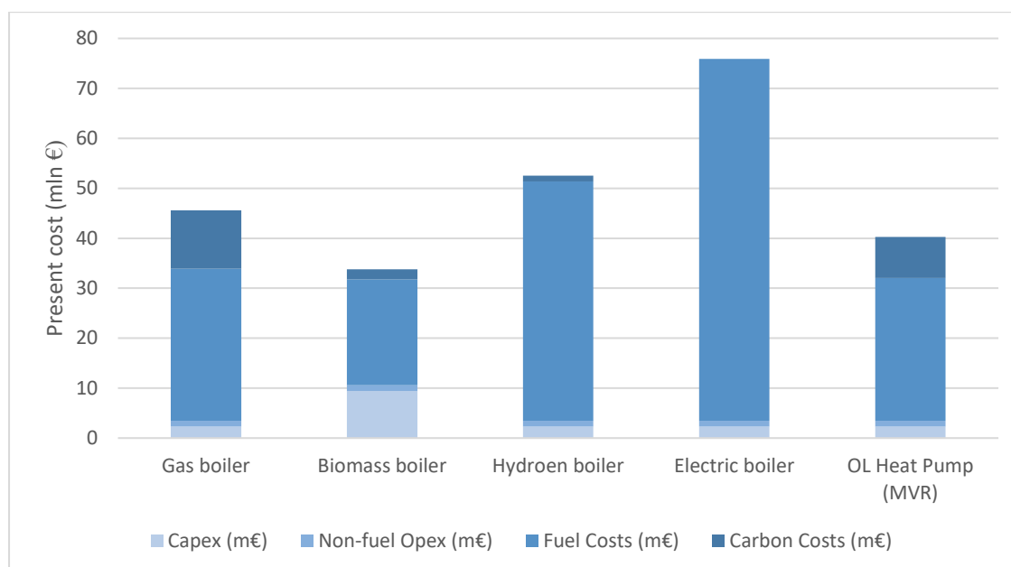
Figure 43: The net present costs of technologies providing low pressure steam 48
